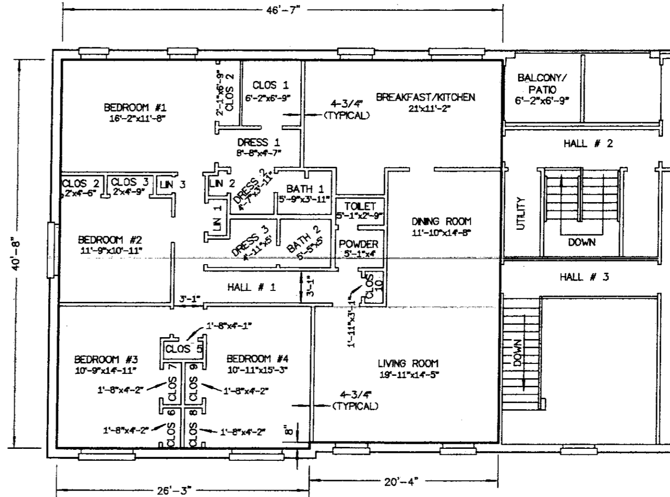
4 BEDROOM FLOOR PLAN SECOND FLOOR BUILDING NO. 1 (REVERSE)
