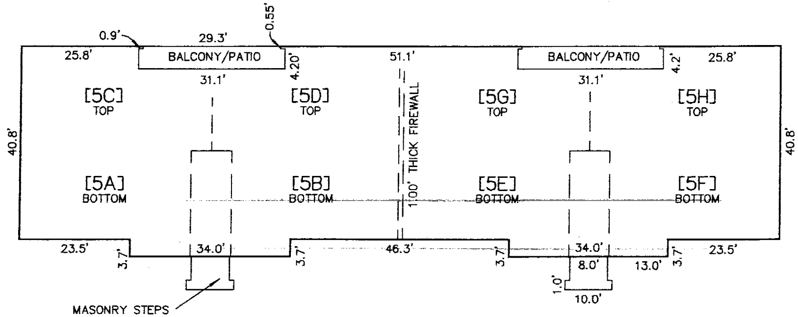
BUILDING NO. 5 FLOORPLAN 3 BEDROOM UNITS
