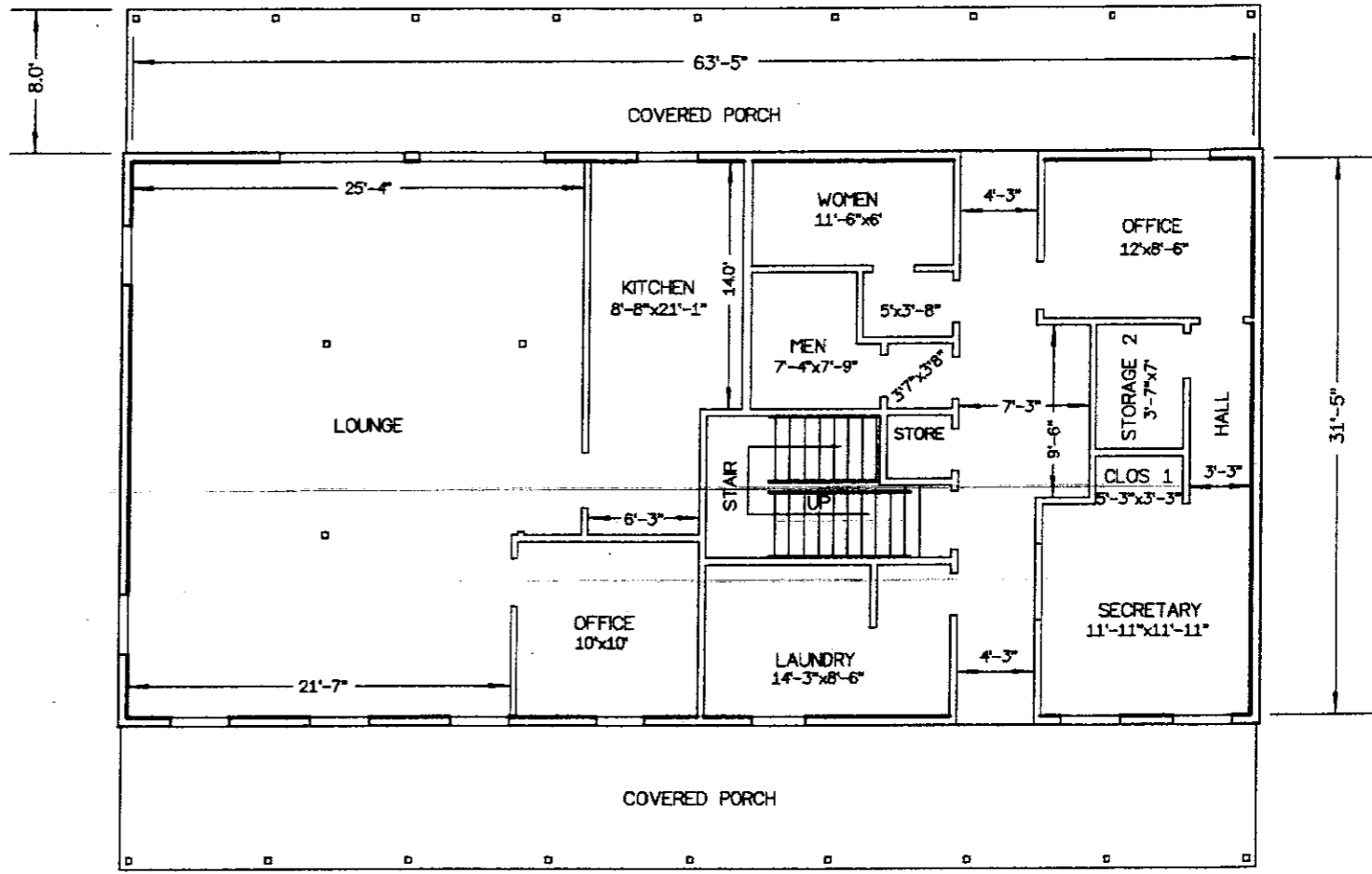
FACILITIES BUILDING FIRST FLOOR
