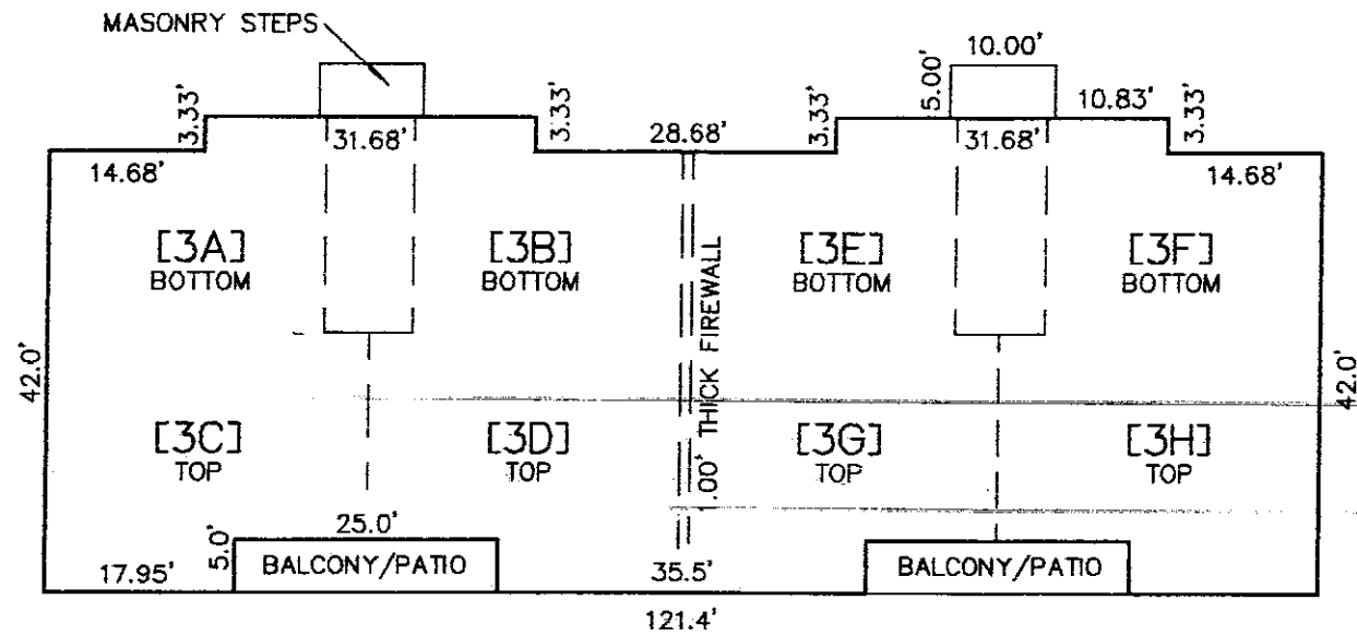
BUILDING NO. 3 FLOORPLAN 2 BEDROOM UNITS
