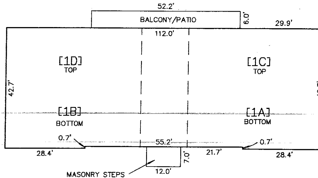
BUILDING NO. 1 FLOORPLAN 4 BEDROOM UNITS
