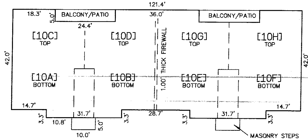
BUILDING NO. 10 FLOORPLAN 2 BEDROOM UNITS
