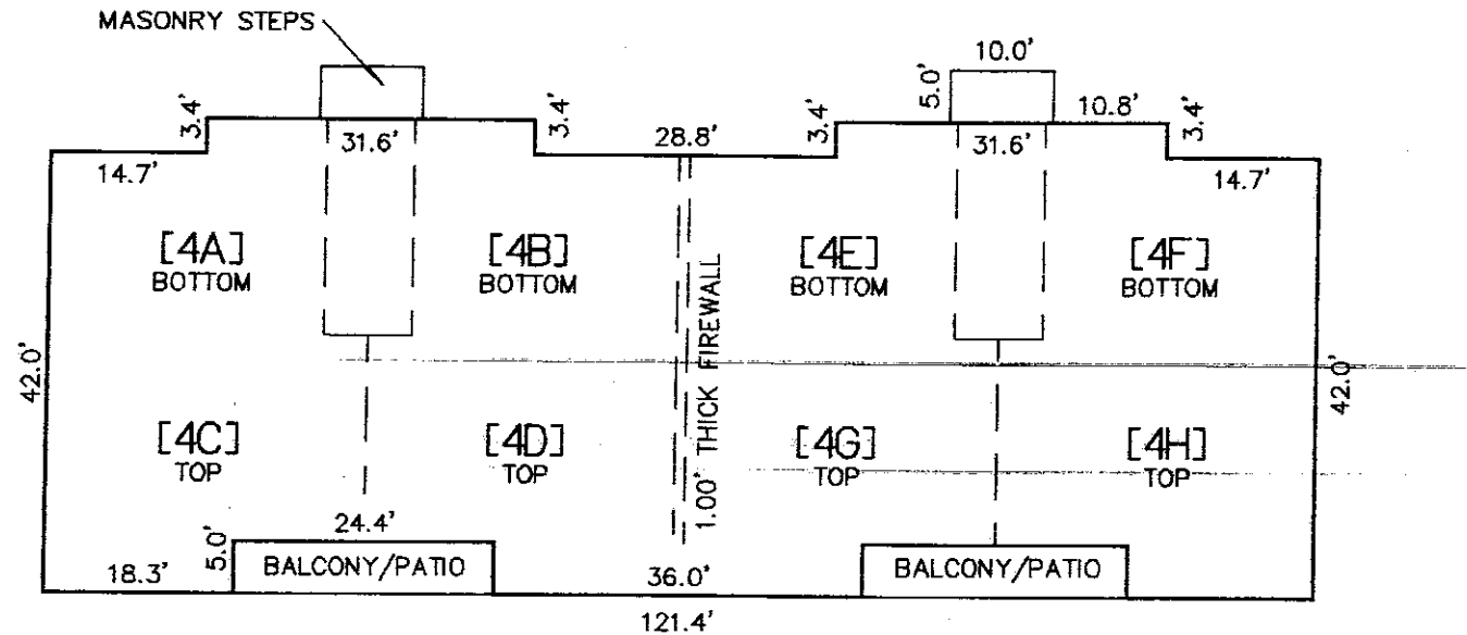
BUILDING NO. 4 FLOORPLAN 2 BEDROOM UNITS
