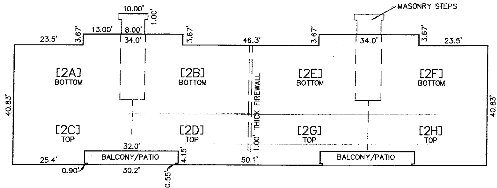
BUILDING NO. 2 FLOORPLAN 3 BEDROOM UNITS
