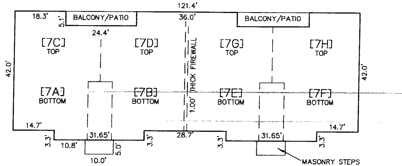
BUILDING NO. 7 FLOORPLAN 2 BEDROOM UNITS
