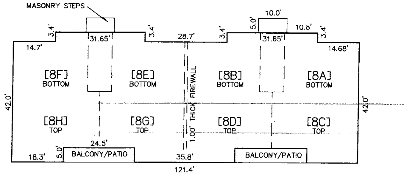
BUILDING NO. 8 FLOORPLAN 2 BEDROOM UNITS
