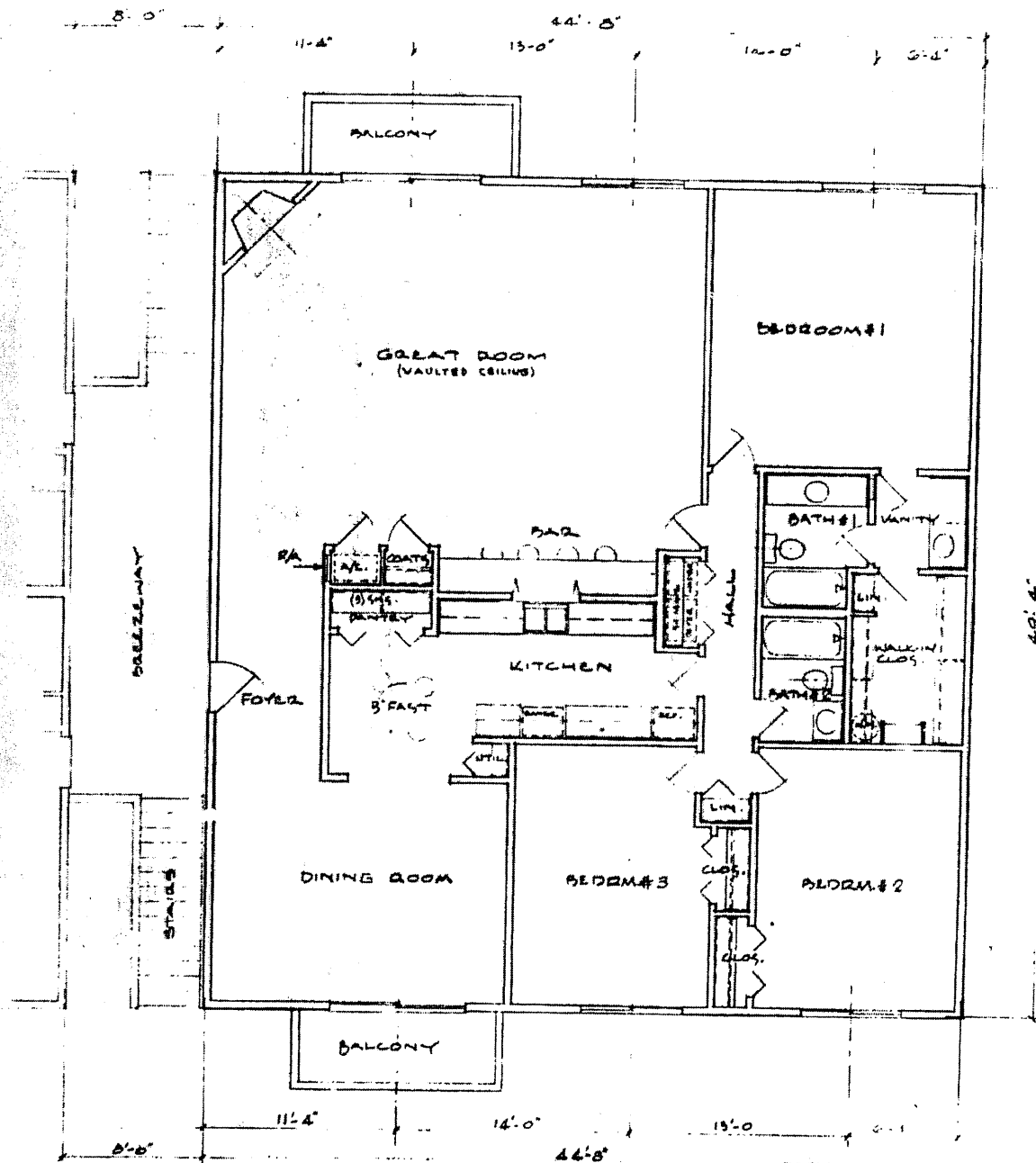
(3) BEDROOM APARTMENT (1) REQ'D. ON 2ND FL. BLDG. "B" EAST END 1/4" = 1'-0" 2.00
